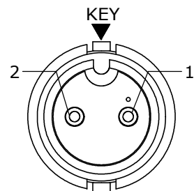
FACE VIEW 6282-2PG-5XXW
