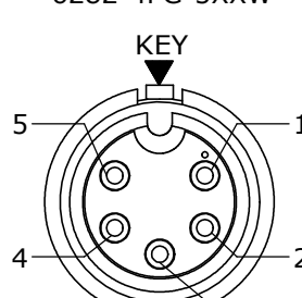
FACE VIEW 6282-5PG-5XXW
