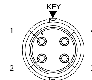
WIRE VIEW 6282-4PG-5XXW SHOWN
