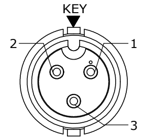
FACE VIEW 6282-3PG-5XXW
