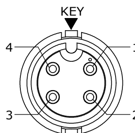
FACE VIEW 6282-4PG-5XXW
