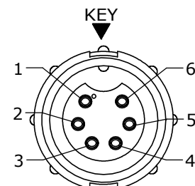
FACE VIEW ASSY: 5280-6SG-5XX
