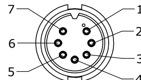
FACE VIEW P/N: 3280-7SG-5XXW
