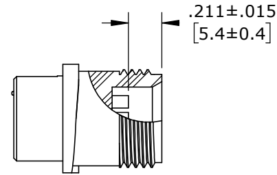
CONTACT HEIGHTS FOR CUSTOMER REFERENCE
