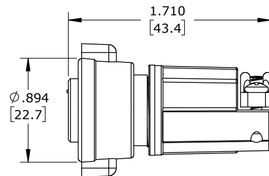
ASSEMBLED VIEW FOR CUSTOMER REFERENCE
