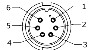
FACE VIEW P/N: 3280-6SG-5XXW
