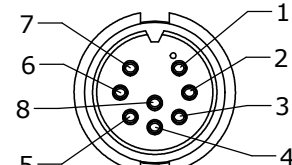
FACE VIEW P/N: 3280-8SG-5XXW
