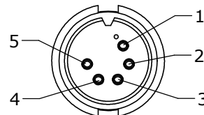
FACE VIEW P/N: 3280-5SG-5XXW
