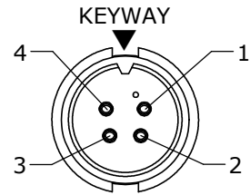
FACE VIEW P/N: 3280-4SG-5XXW
